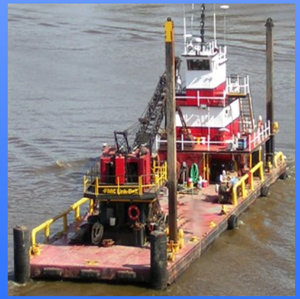
Self Propelled Work Barge
